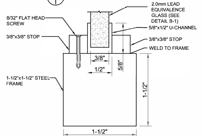
C SECTION AT FRAME
