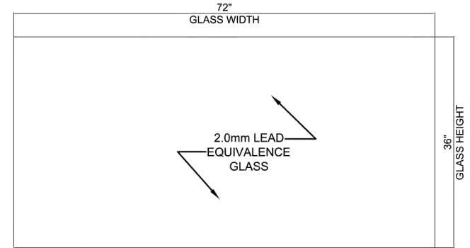
B 1 GLASS ELEVATION
