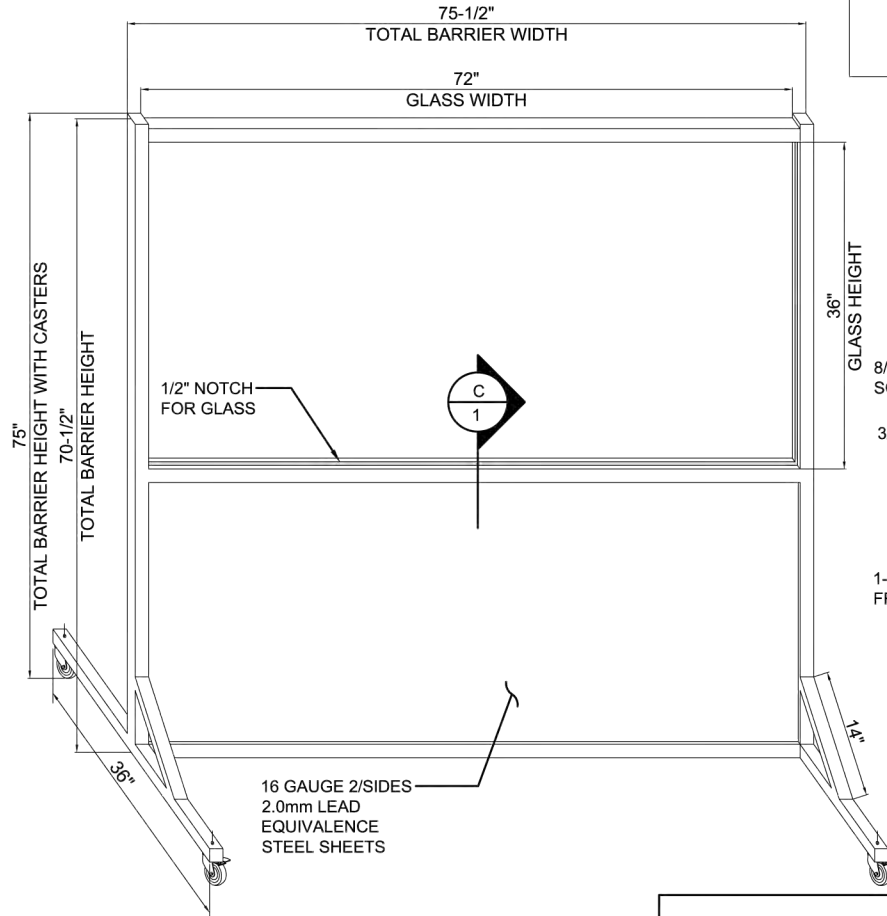
A 1 BARRIER ELEVATION
