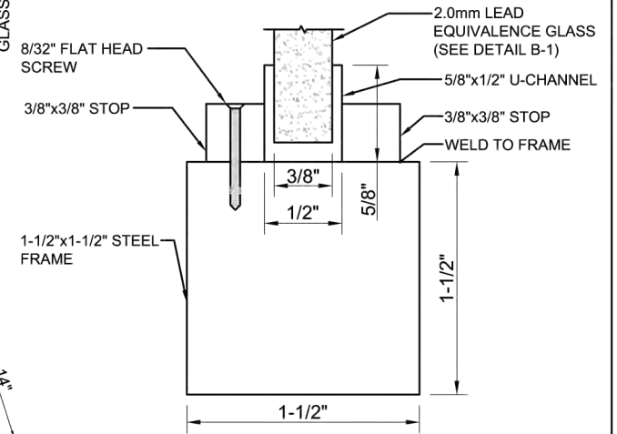
C 1 SECTION AT FRAME
