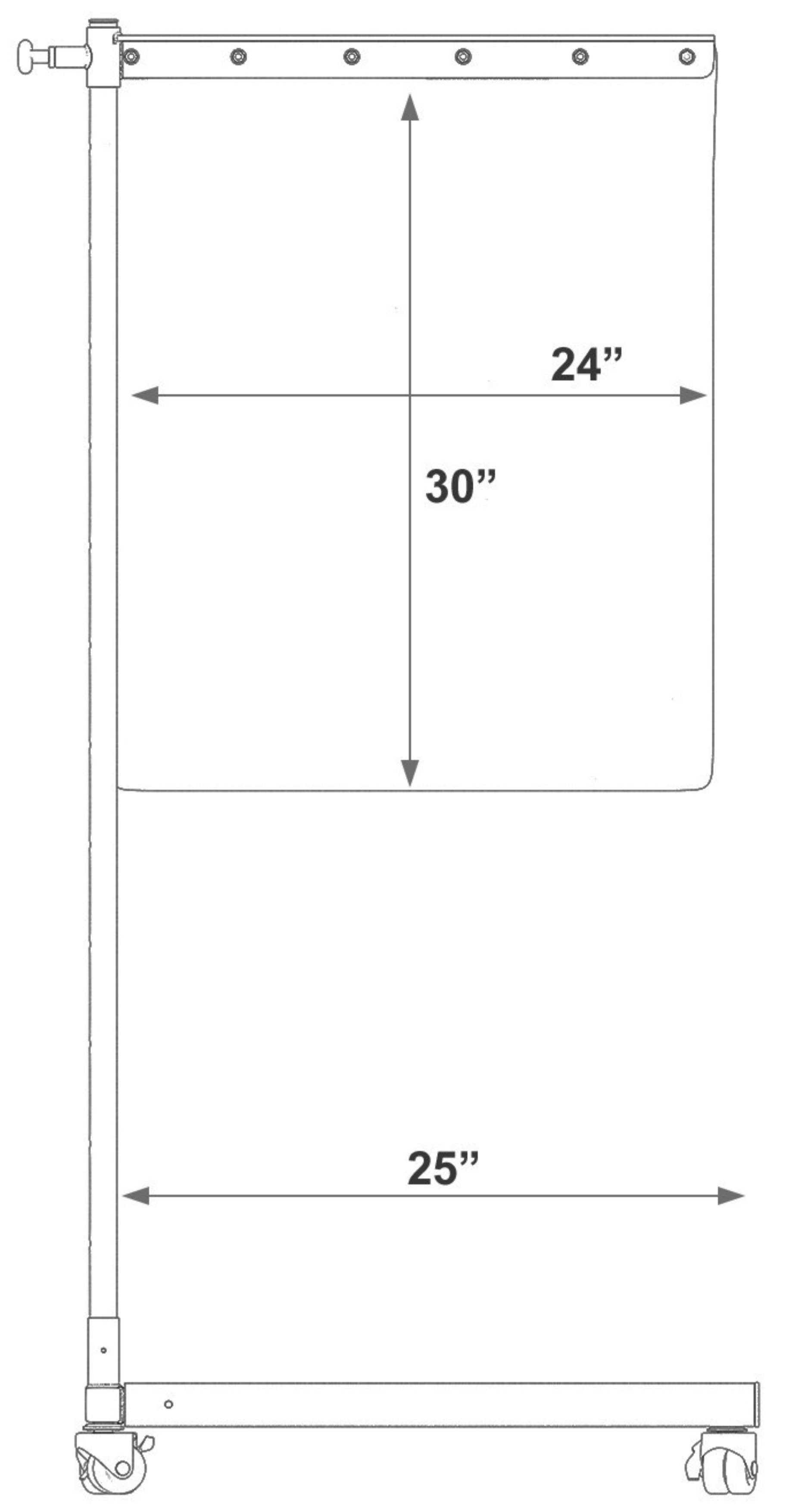
RIGHT VIEW
