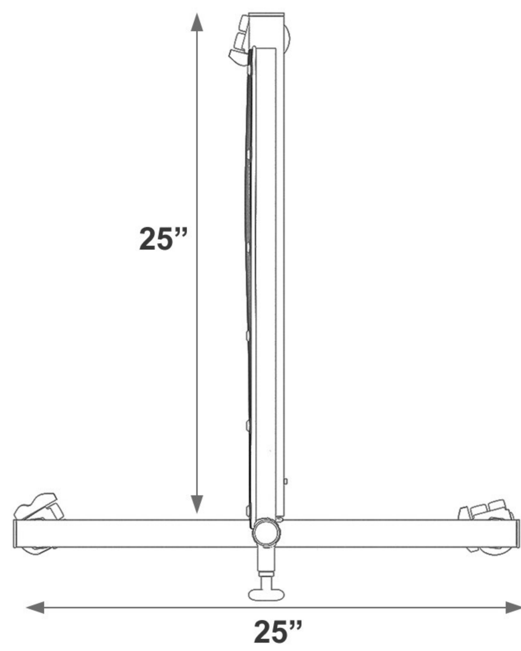
TOP VIEW
