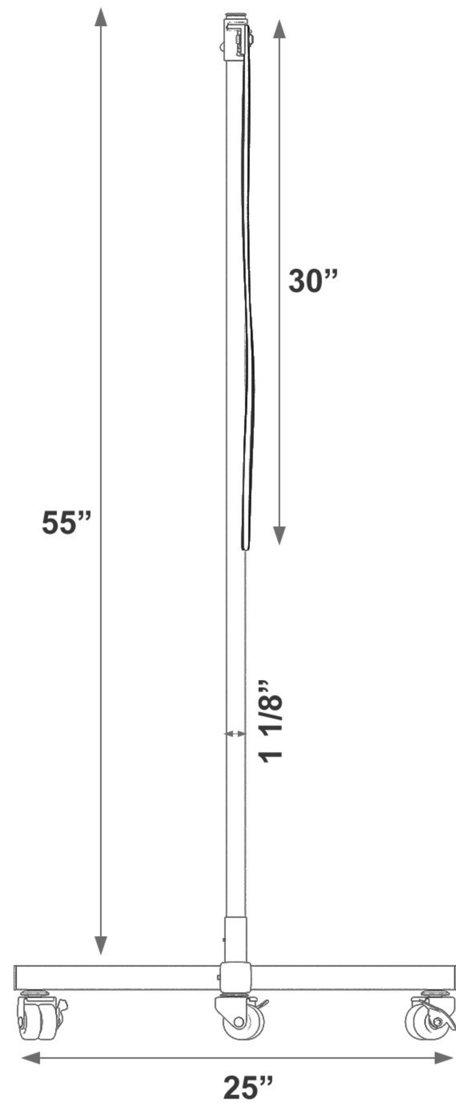
FRONT VIEW
