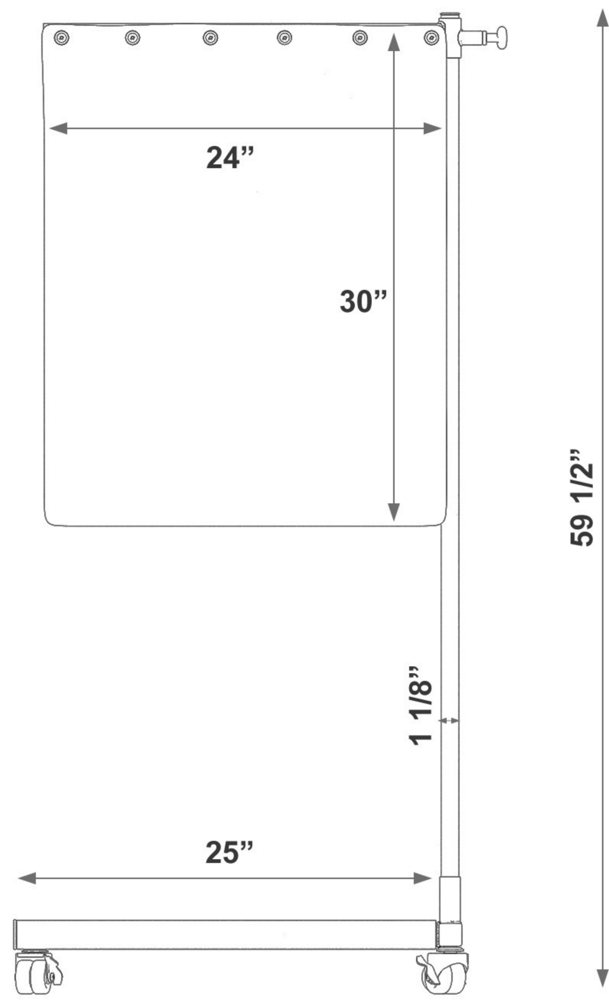
LEFT VIEW
