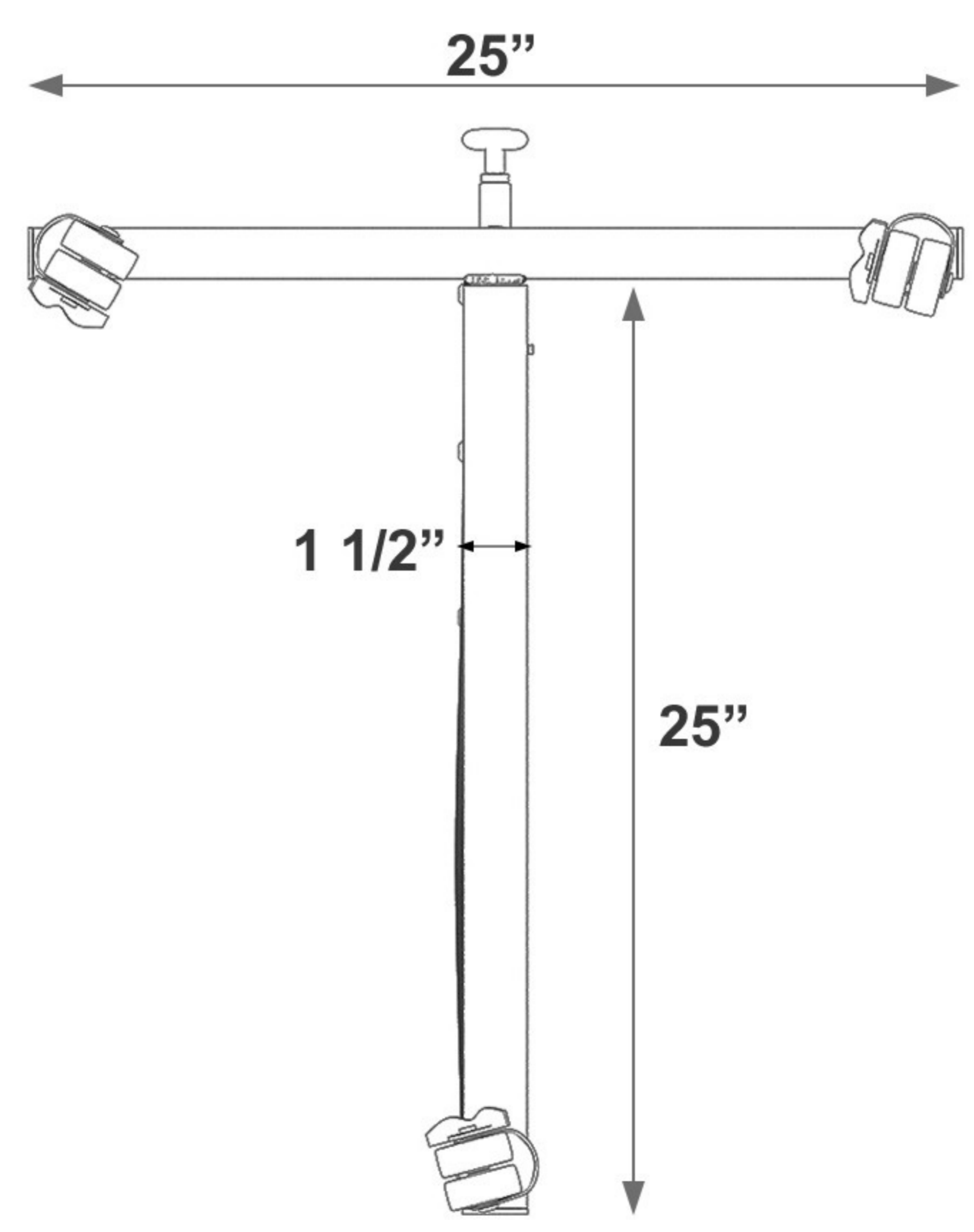
BOTTOM VIEW
